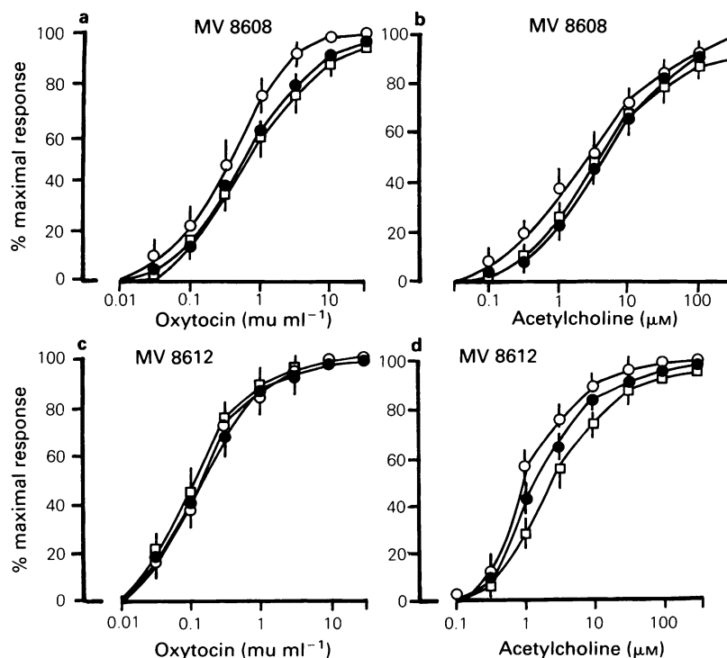
Figure 5 Mean concentration-response curves for oxytocin (a and c) and acetylcholine (b and d) in the isolated uterus of the rat. Control responses (○) and responses in the presence of compounds MV 8608 (a and b) or MV 8612 (c and d), ( \mu\text{g ml}^{-1} ): 10 (●) and 20 (□). Each point represents the mean of 4 to 5 experiments and the vertical lines indicate the s.e.mean.
